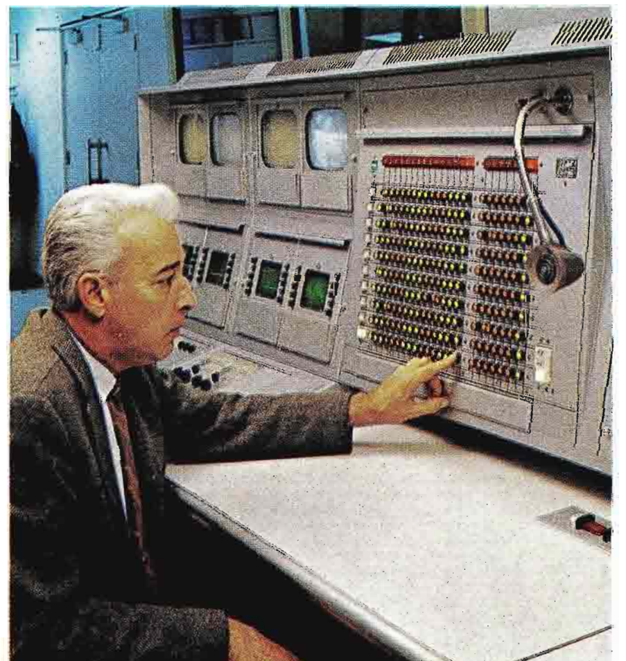
STATION BREAK AUTOMATION section houses TSA-3 panel capable of handling 15 video and 7 audio inputs in a preset sequence of ten events. Panel at the operator's right includes remote control of sync generators and stabilizing amplifiers.
