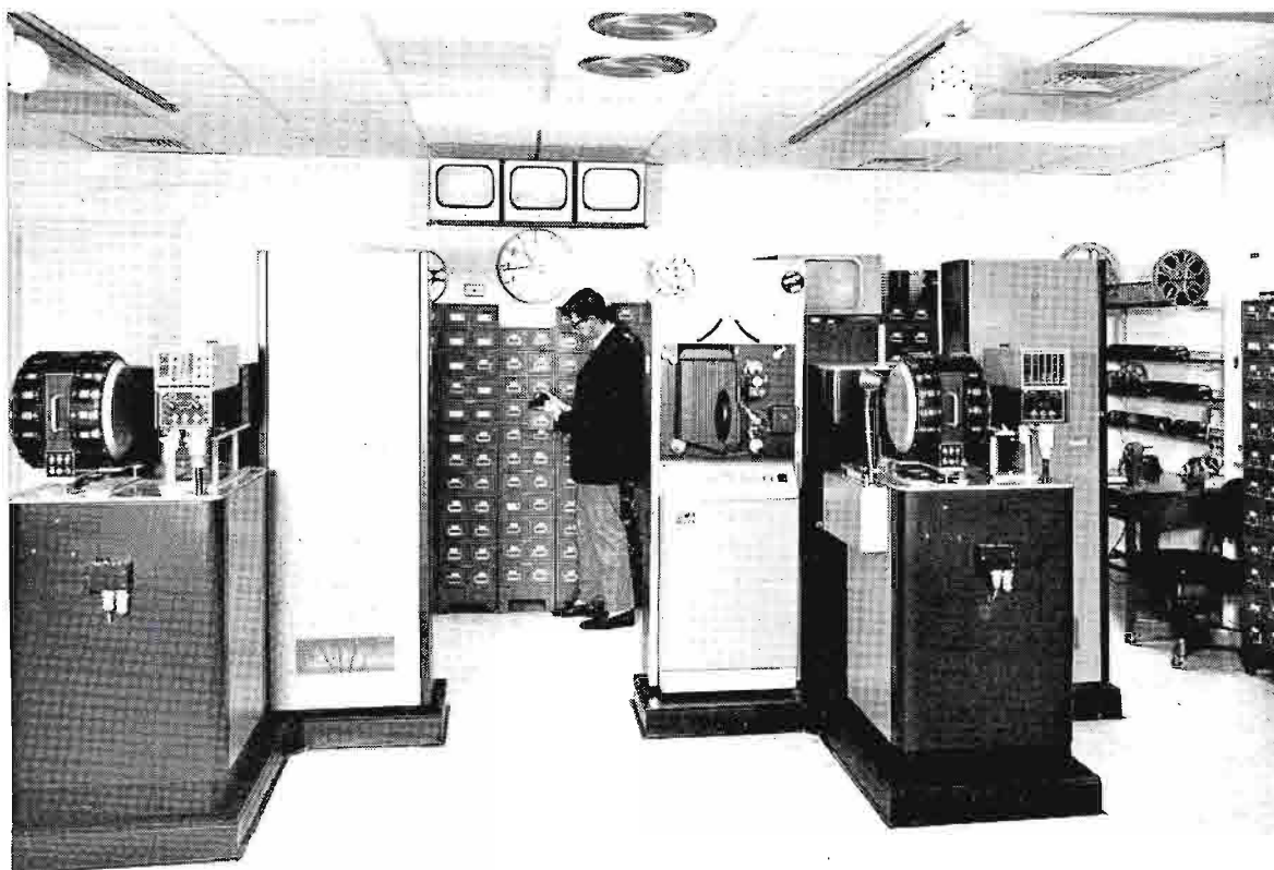
FILM AREA includes two film islands, storage and film editing facilities. Latest-design equipments for color and monochrome include a TK-27 4-vidicon color film chain and two TK-22 monochrome film chains.
