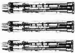
4½-inch I.O. in luminance channel; three vidicons in chrominance channels
