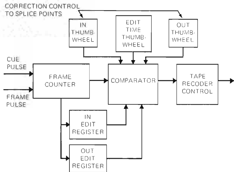
FIG. 2 Simplified block diagram of the TEP system.
