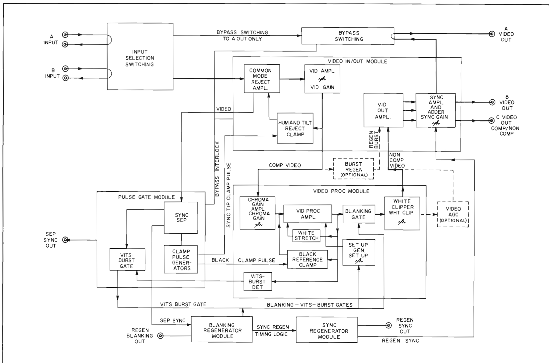
FIG. 8 Block diagram of TA-19 circuits.
