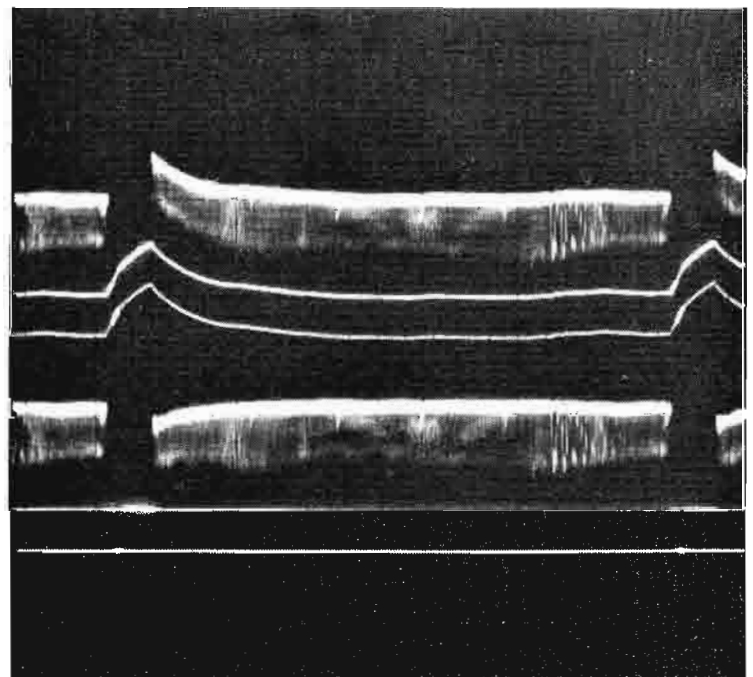
FIG. 3 Waveforms showing how drastic tilt on input signal is cleaned up in the output of the TA-19.
