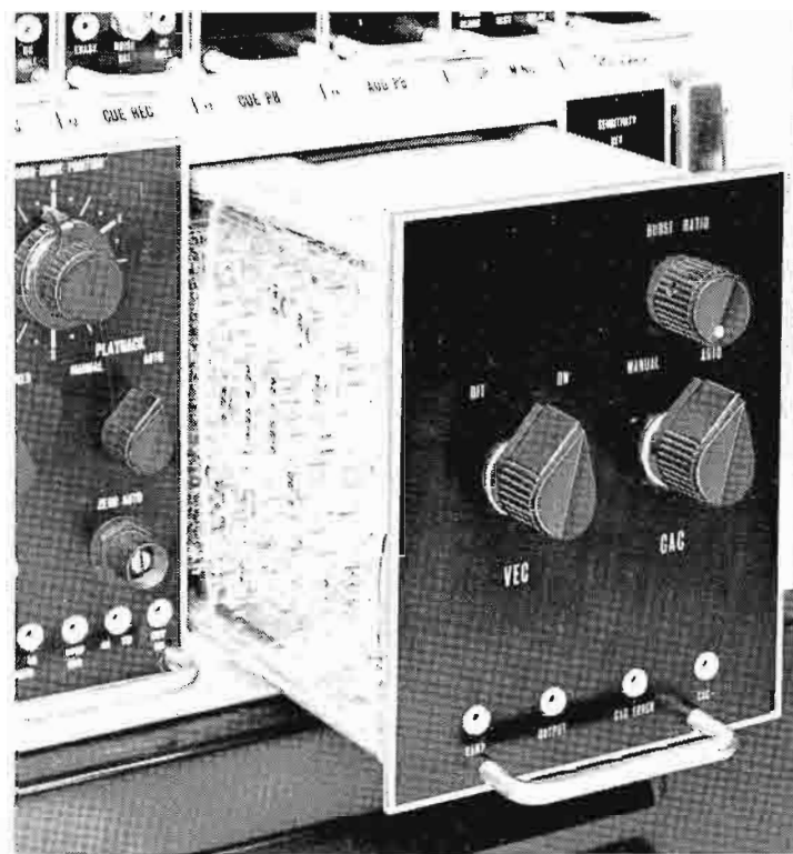
FIG. 9 CAVEC module performs chroma amplitude and velocity error correction on a line-by-line basis, helping operators achieve quality replays, free from banding. The TR-60 is partially prewired for this accessory.
