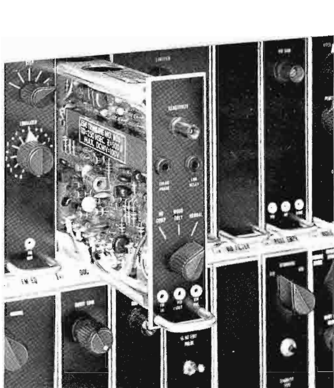
FIG. 8 Dropout compensator module features NTSC corrected color phase insertion and all electronic setup. The TR-60 is prewired for insertion of this plug-in module.
